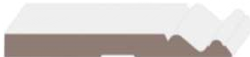
BASEBOARD Stock Code Dimensions B8006 9/16"x5+7+3/8 "
